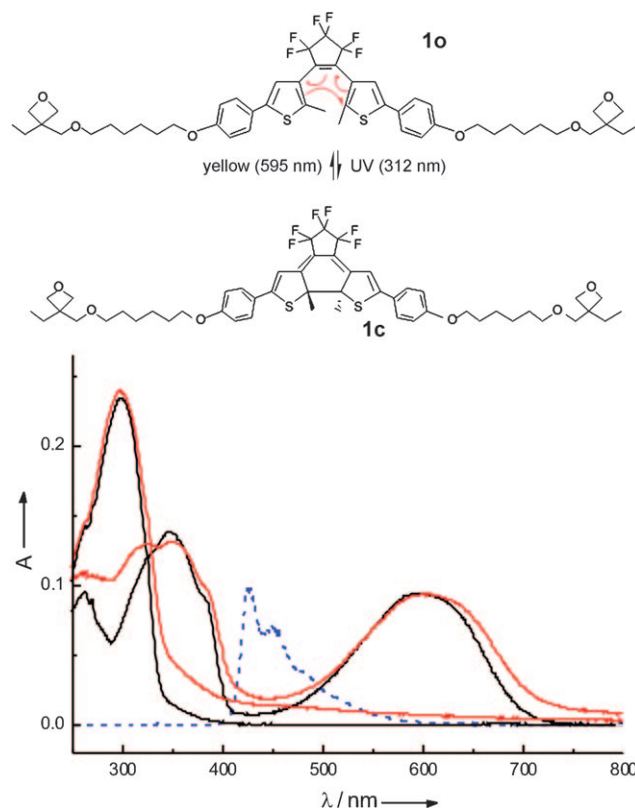
Figure 1. UV/Vis spectra of the colorless open form 1o and the colored closed form 1c : 2.5 \times 10^{-6} M solution in CH 2 Cl 2 (—), 40 nm crosslinked film on glass (—); electroluminescence spectrum of the photoswitchable device with B as emissive layer (---, arbitrary units).
